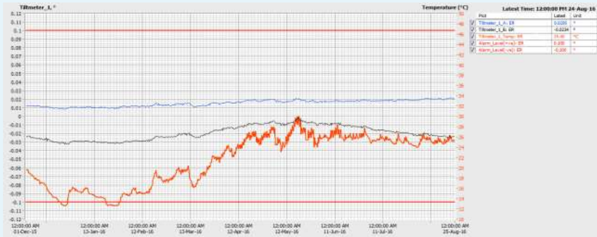
Fig. 5 : Screen Shot of Graph Presented by a Cloud Based Data Monitoring Service Showing Eight Months Data of a Biaxial Tilt Sensor Sampled Once a Day at a Fixed Time. The Trace in Red Showing Larger Variation is of Ambient Temperature Variation. The other Two Traces are Magnitude of Tilt in Degrees Along Two Orthogonal Axes. The Difference Between the Maximum and Minimum Value of Tilt Registered is Approximately 0.02 Degrees. The Two Red Lines at the Top and Bottom are Alarm Limits set for the Biaxial Tilt Sensor.
