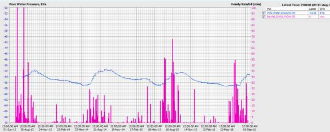
Fig. 7 : Shows Three Year's Data of Changes in Ground Water Table and Rainfall. Ground Water Level is Logged Four Times a Day. Rainfall is Logged Continuously. Data is Transmitted Once a Day to Cloud Server. Co-Relation of Variation in Ground Water Level with Rainfall can be seen on the Graph. Similar Instrumentation is used for Online Automatic Monitoring of River Water Level and Rainfall with Time.
