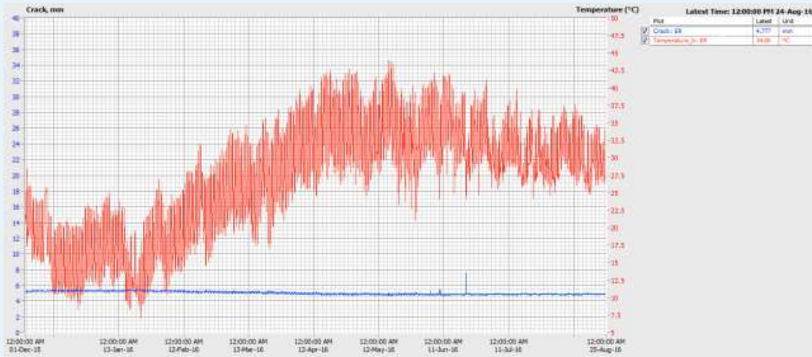
Fig. 6 : Shows Eight Months Data of Crack Meter Set at 6 MM to Register Both Closing and Opening of Crack with Time. Band Like Trace is Ambient Temperature. as Sensor is Being Sampled Every 30 Minutes it is Tracking Variation In Ambient Temperature Over Whole Day Unlike Figure 5 in which Sensor is Sampled Once A Day.
