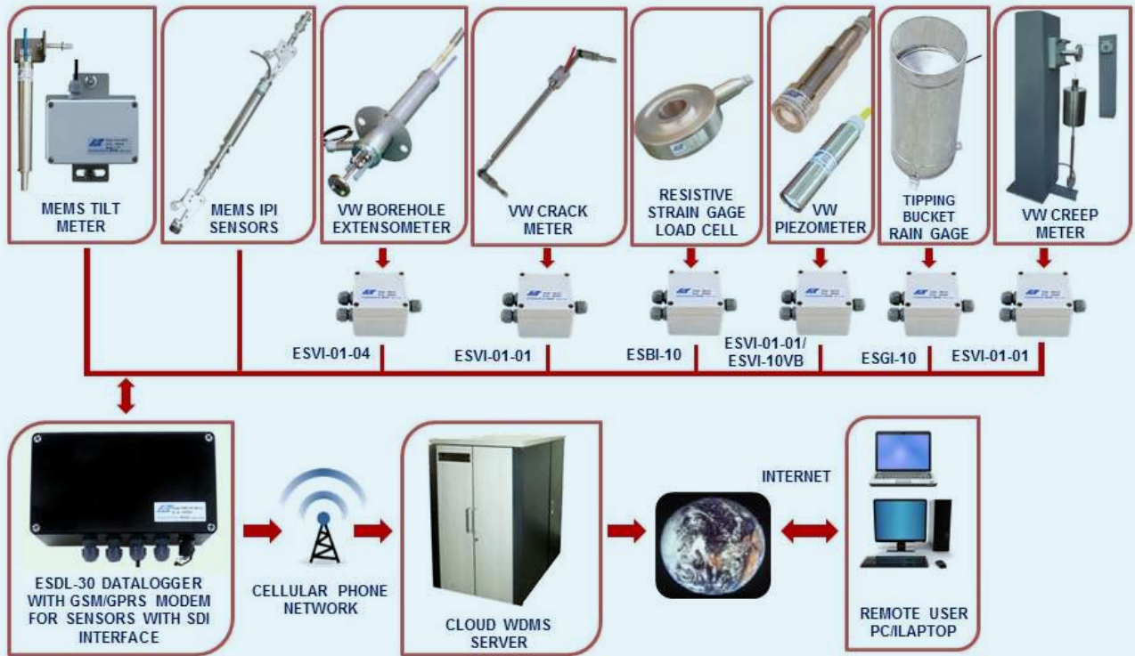
Fig. 3 : Different Sensors Connected through SDI-12 Bus Cable to a Data Logger with Web Based Data Monitoring
